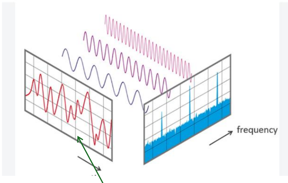
Figure 3: Interpret this as follows: The signal is sum of three sine-waves, each one of fixed frequency. There may be multiple frequencies of very low-amplitude also.
